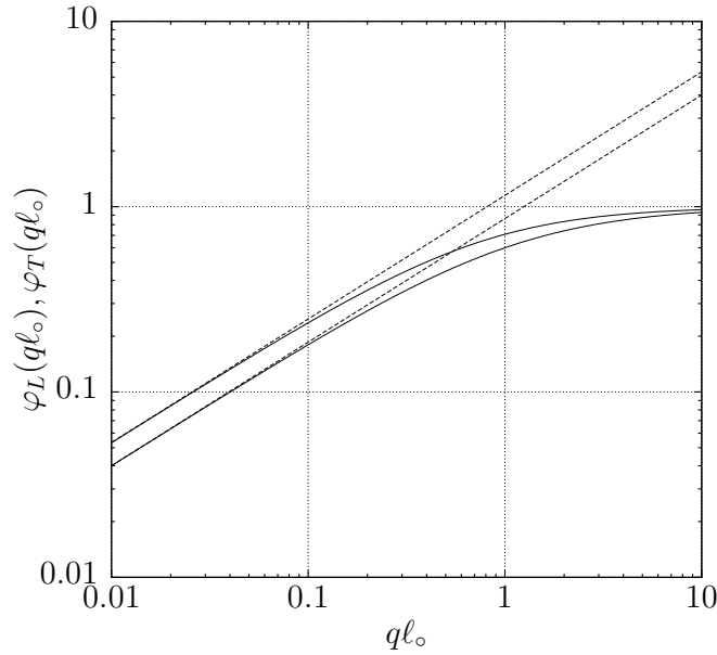
Figure 5: The functions \varphi_L(q\ell_0) and \varphi_T(q\ell_0) , based on the von Kármán spectrum. For values of q\ell_0 up to about 0.1 we are in the domain of local isotropy, where both functions are proportional to (q\ell_0)^{2/3} .
